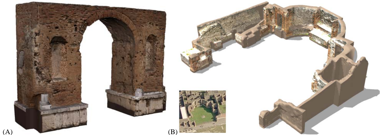
(A) Figure 5: 3D model of the Nero Arch (10m x 2.5 m x 7.5m) produced from the acquired range data and textured with digital images for photo-realistic visualization (A). Photo-realistic range-based 3D model of the Lari's temple (27m x 27m x 6m ). In the left-lower corner an image of the temple from an oblique aerial view (B).
